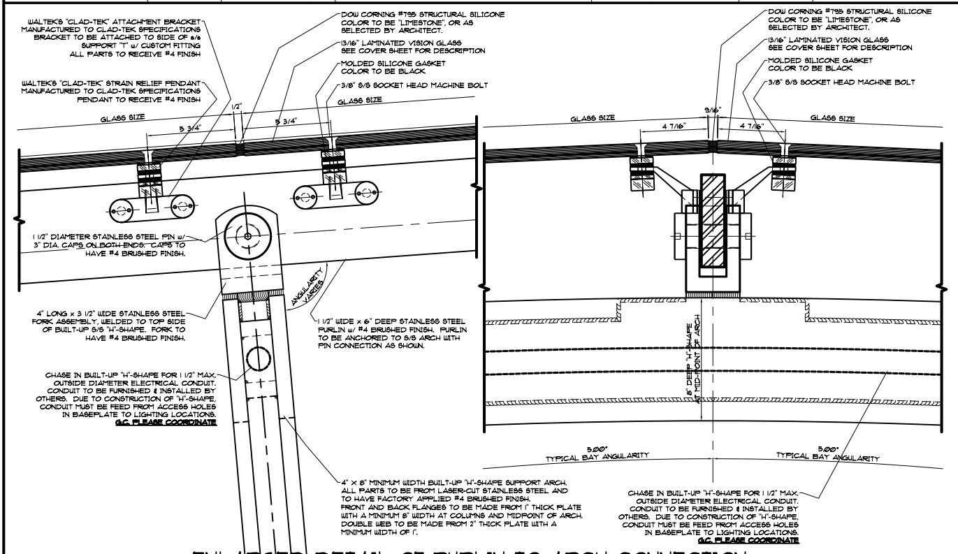
ENLARGED DETAIL OF FURLIN TO ARCH CONNECTION
