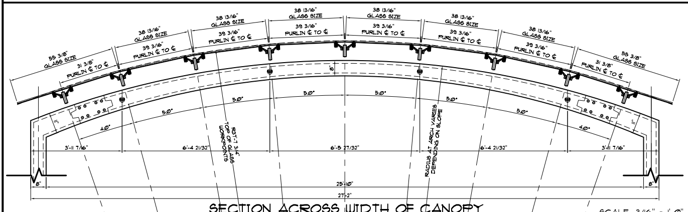
SECTION ACROSS WIDTH OF CANOPY
