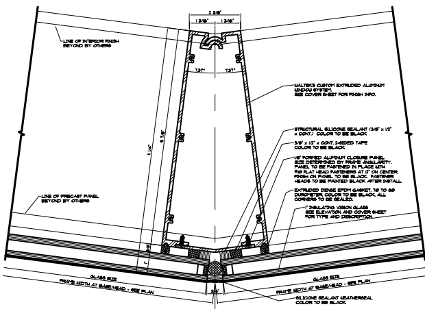
A INTERMEDIATE MULLION DETAIL SCALE: 2" = 1'-0"
