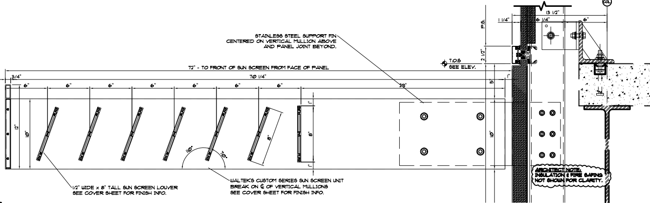
C DETAIL CUT AT SUNSHADE
