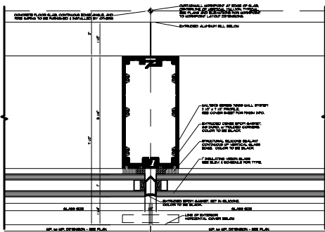
A HEAD DETAIL
