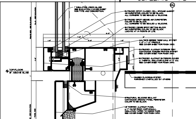
B MIDDLE FIN ATTACHMENT
