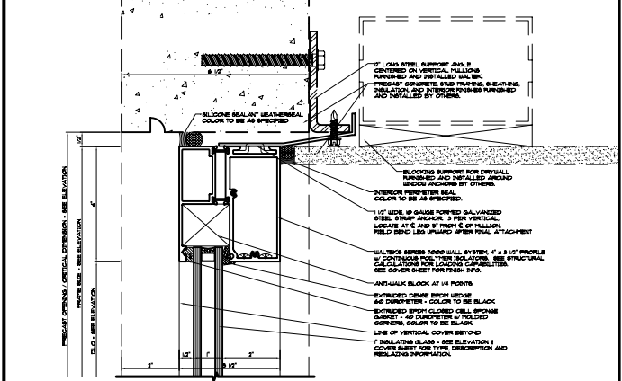
A TYPICAL HEAD DETAIL
