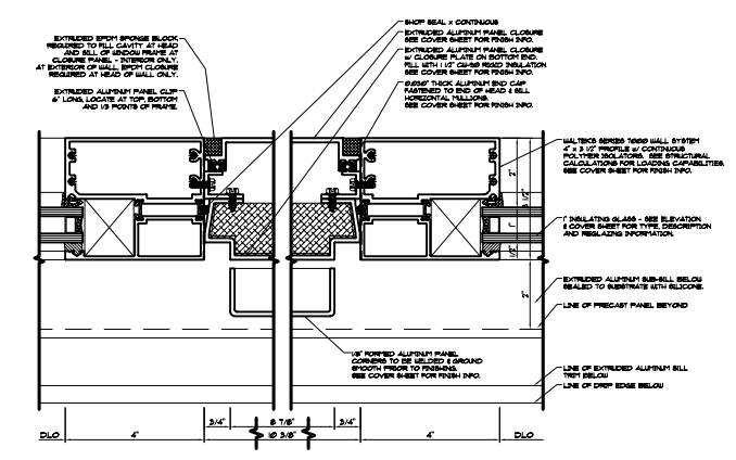
B VERTICAL AT PANEL
