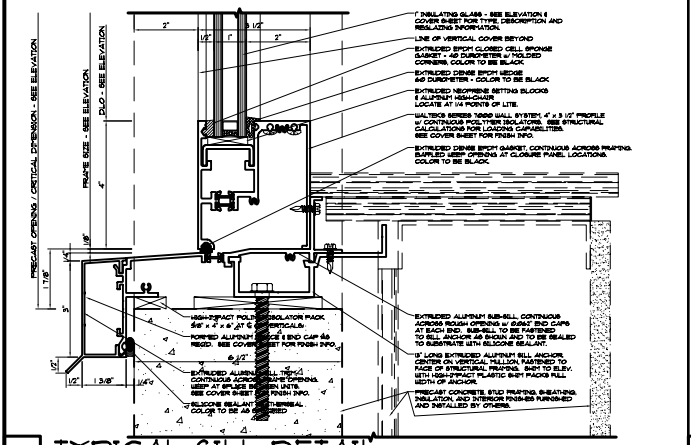
C TYPICAL SILL DETAIL
