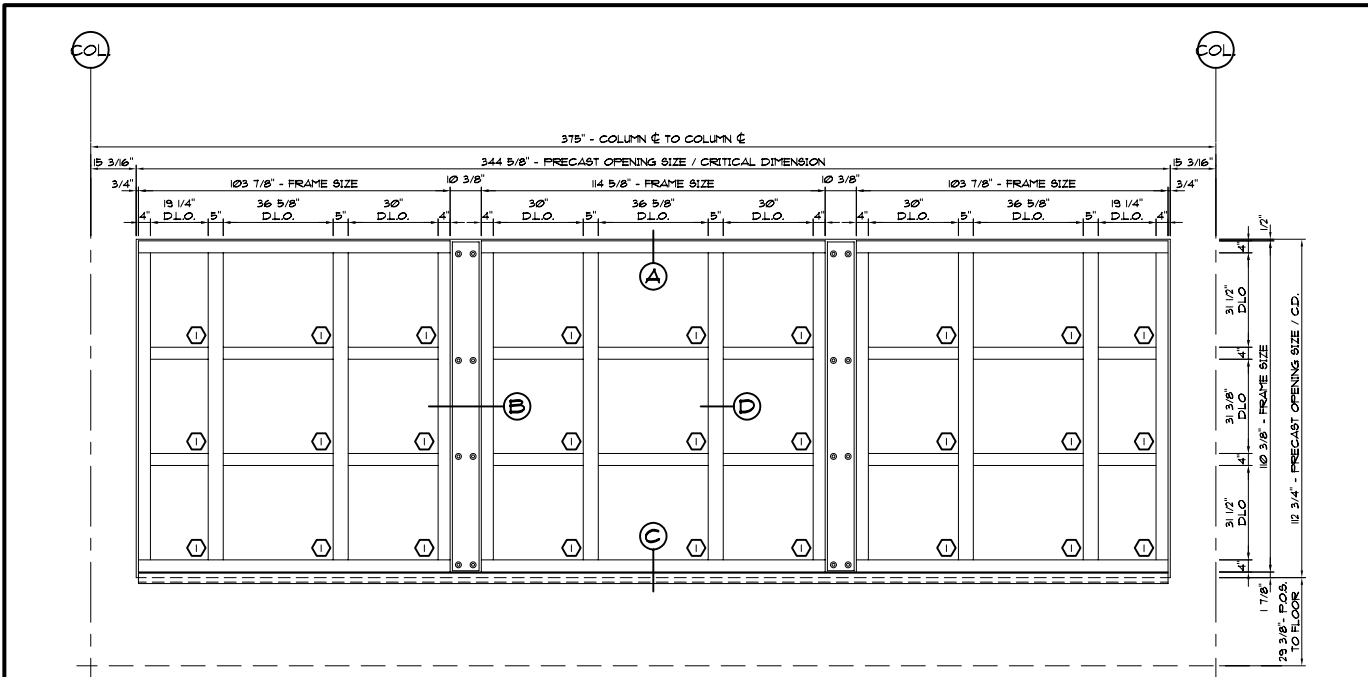
TYPICAL WINDOW ELEVATION
