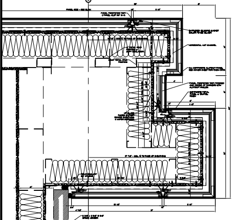
B PANEL JAMB DETAIL SCALE: 1/2" = 1'-0"
