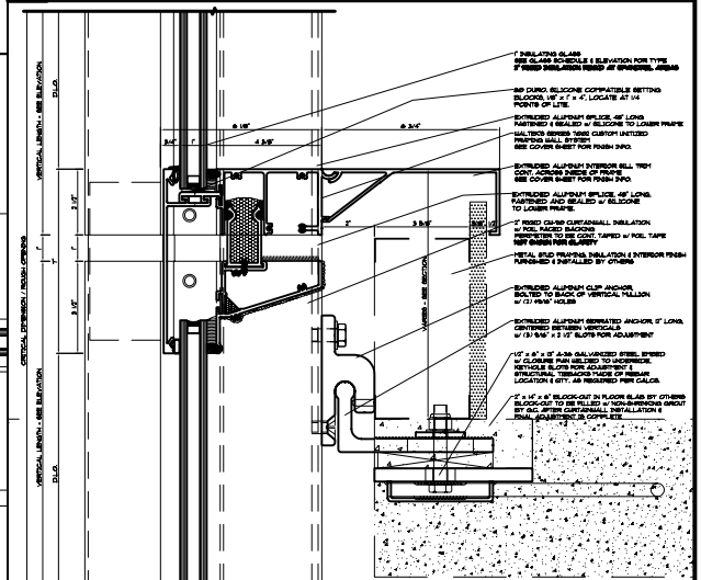
D HORIZONTAL AT SLAB SCALE: 1 1/2" = 1'-0"
