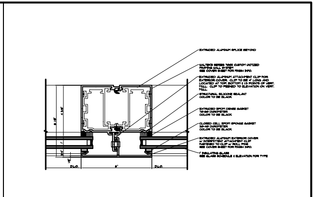
A VERTICAL MULLION SCALE: 1 1/2" = 1'-0"
