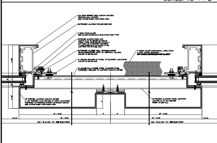
E JAMB AT COLUMN PANEL SCALE: 1 1/2" = 1'-0"
