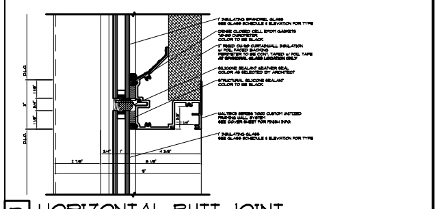
B HORIZONTAL BUTT-JOINT SCALE: 1 1/2" = 1'-0"
