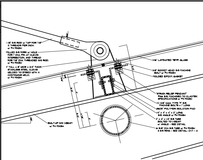
DETAIL AT CLEVIS ATTACHMENT
