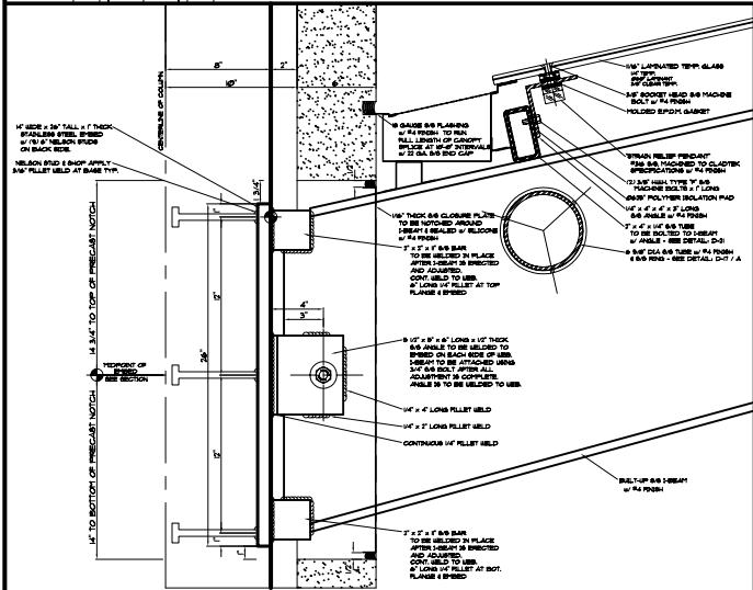
DETAIL AT COLUMN ATTACHMENT
