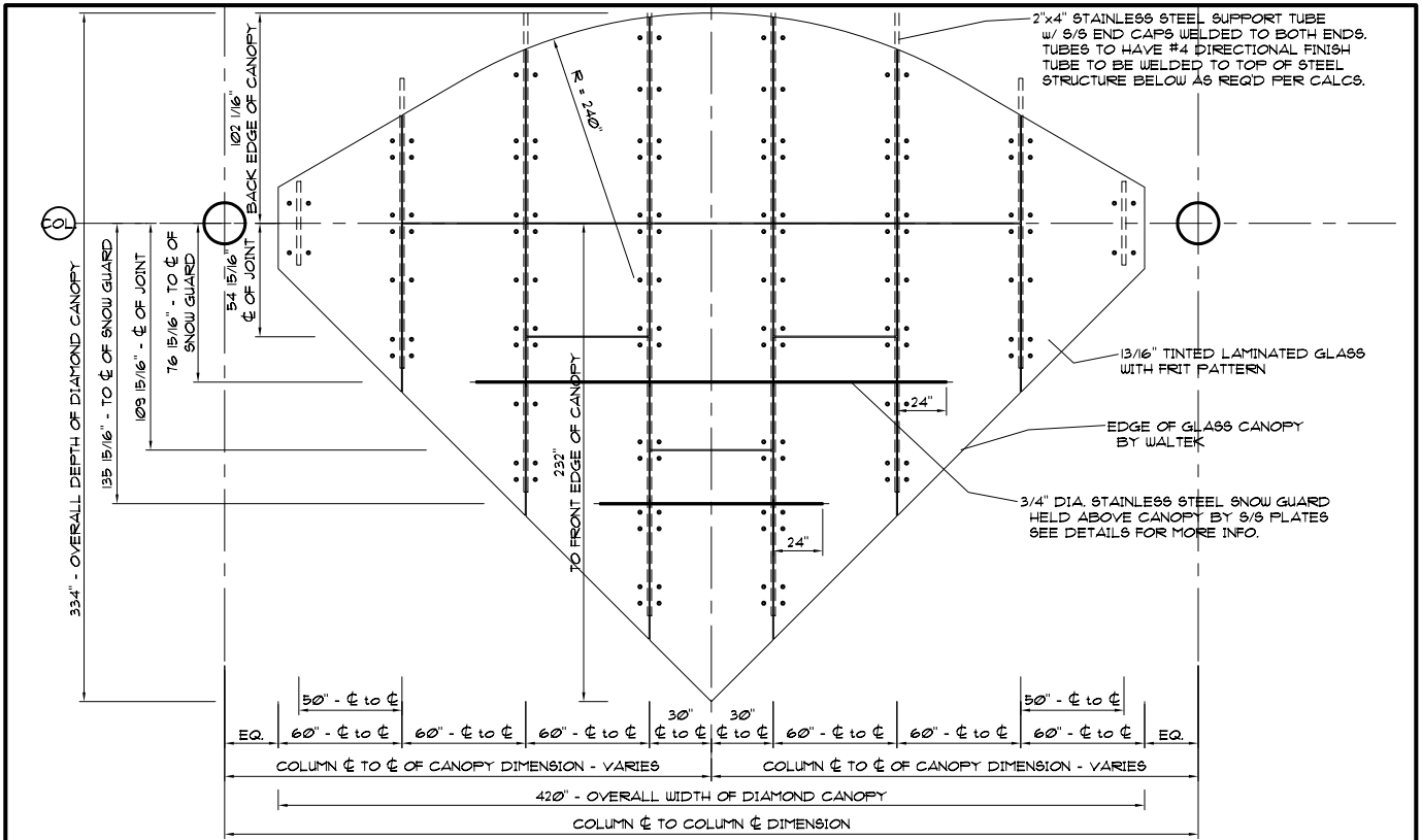
PLAN AT TYPICAL DIAMOND SHAPED CANOPY
