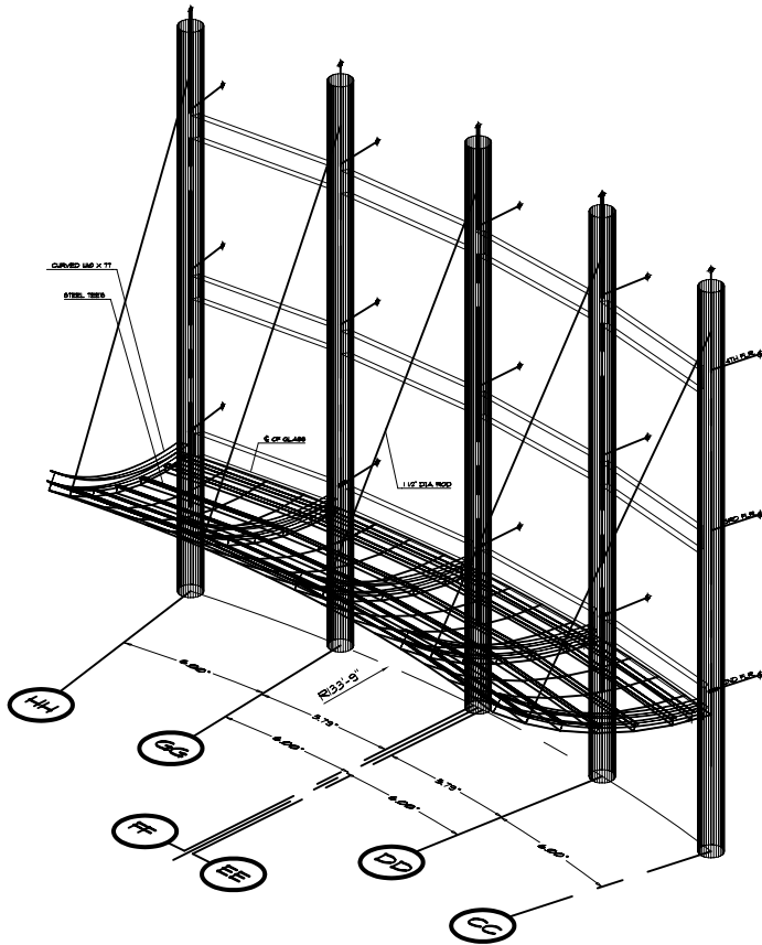
ISOMETRIC OF CANOPY
