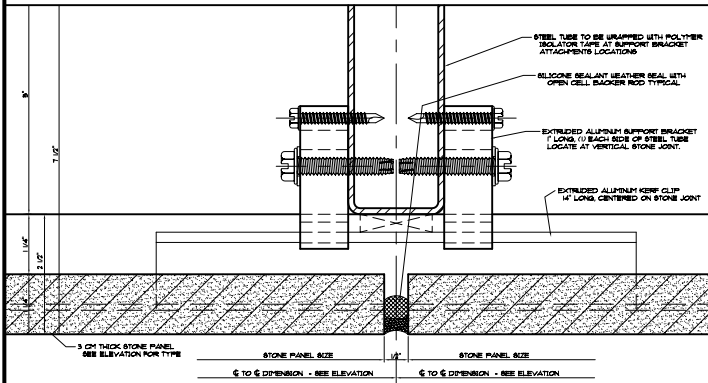
A TYPICAL STONE JOINT DETAIL
