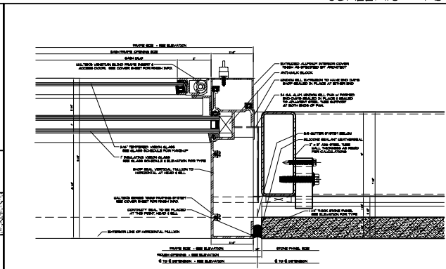
C WINDOW JAMB DETAIL
