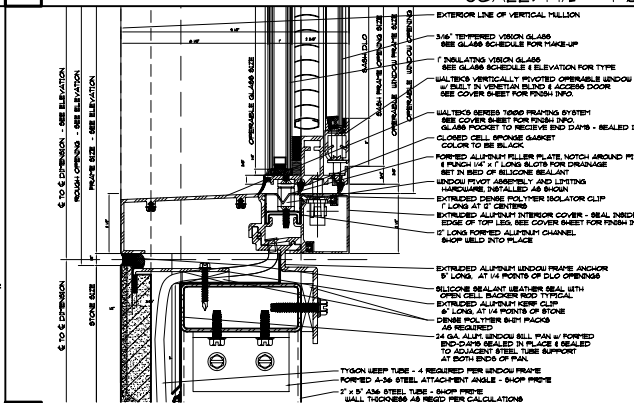
D WINDOW SILL DETAIL
