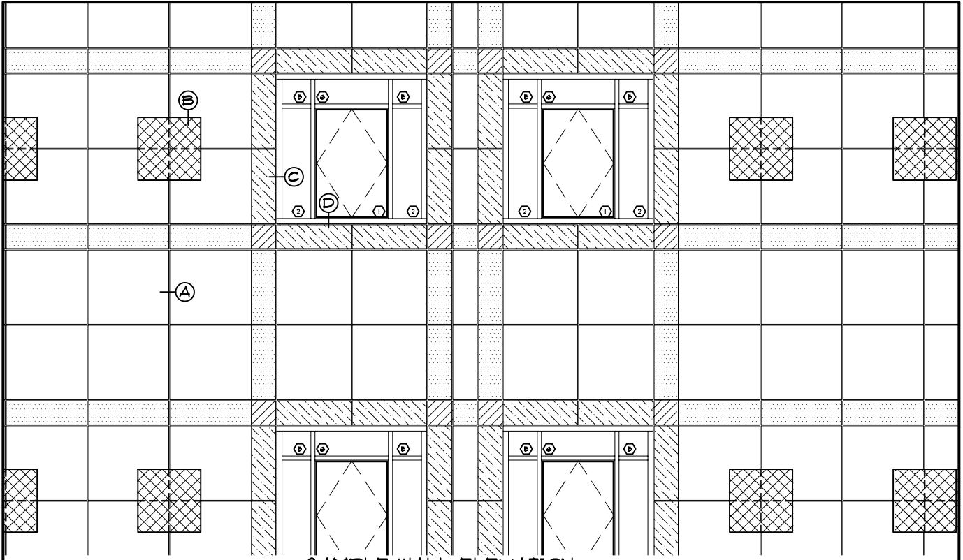
SAMPLE WALL ELEVATION
