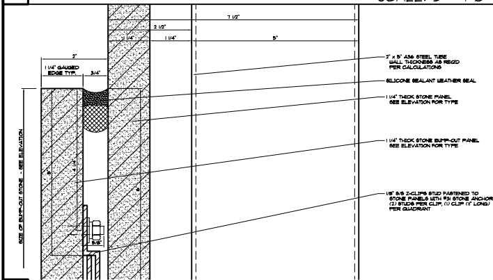
B DETAIL AT ACCENT STONE
