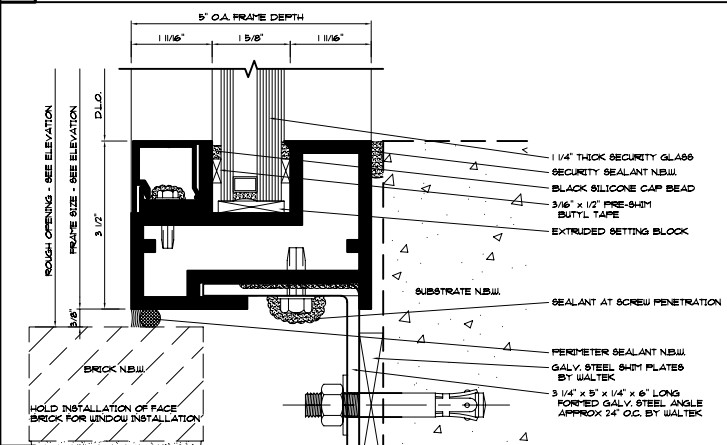
B SILL DETAIL
