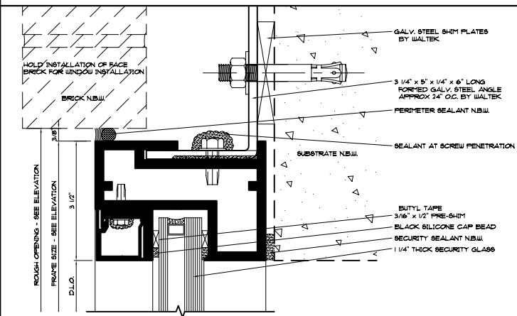
A HEAD DETAIL
